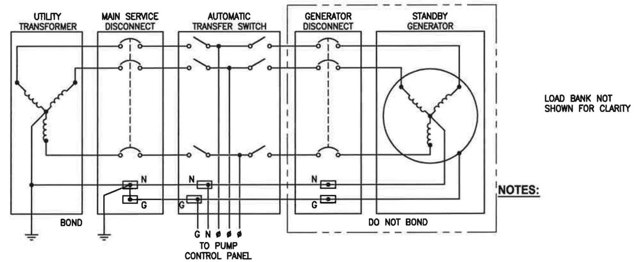
GENERATOR AND TRANSFER SWITCH CONNECTION DIAGRAM
