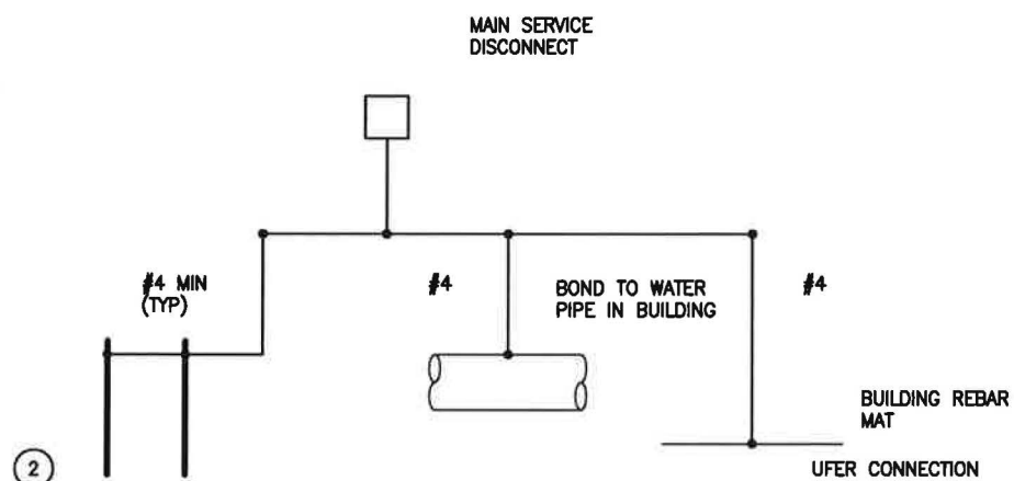
GROUNDING DETAIL
